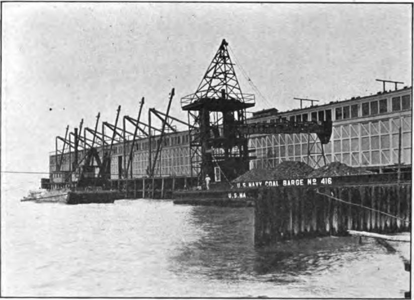
Derricks for supporting De Mayo elevators, Bunkering Depot, Newport News, Va.
