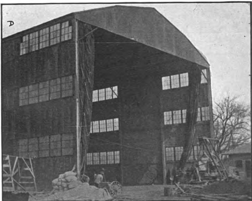
Kite-balloon hangar, Hampton Roads, Va.
