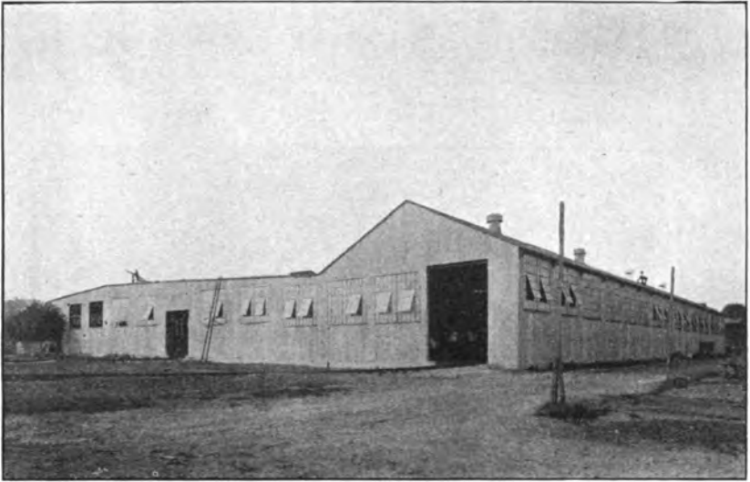
Emergency storehouse, Navy Yard, Philadelphia, Pa.
