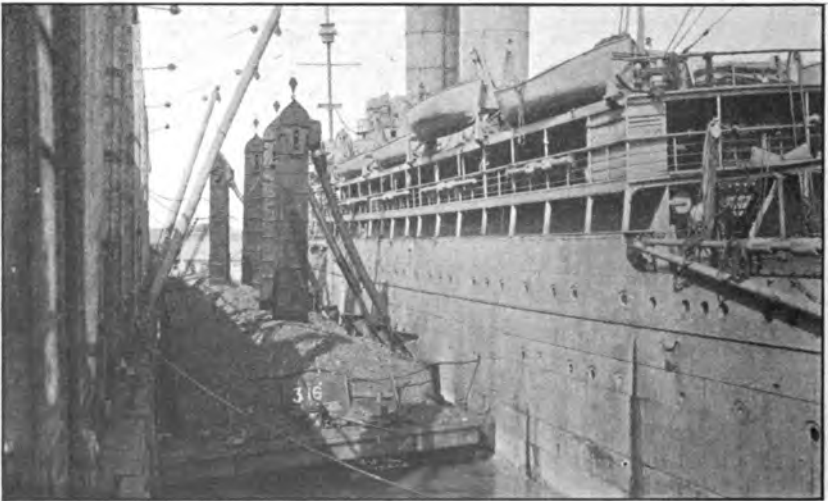
De Mayo elevators in operation at Bunkering Depot, Newport News, Va.
