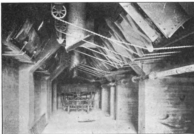
Ash-removal system at power plant, Navy Yard, Philadelphia, Pa.
