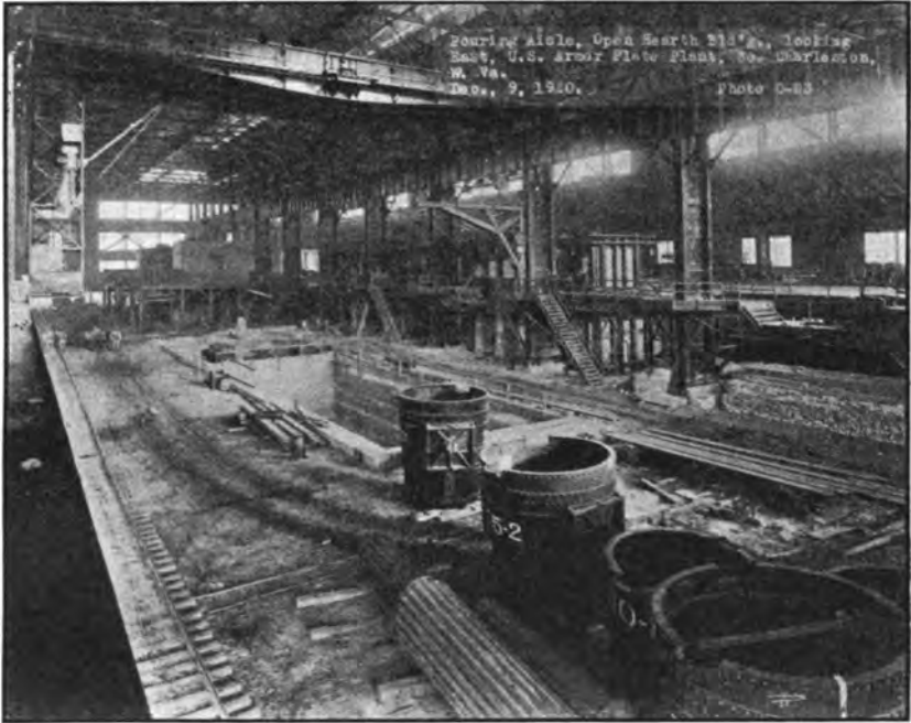
Pouring aisle in open-hearth building, Armor Plant, Charleston, W. Va.
