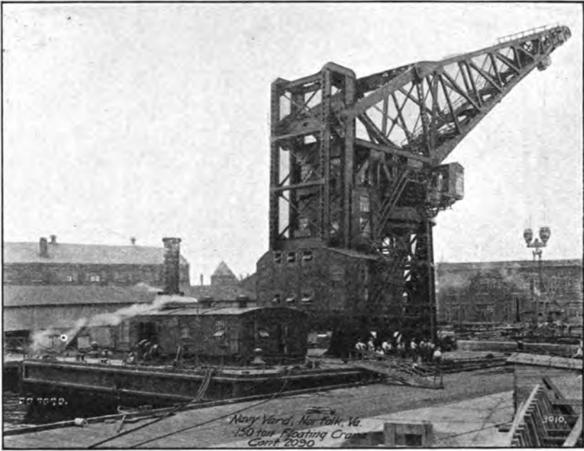
Floating crane (150-ton), Navy Yard, Norfolk, Va.
