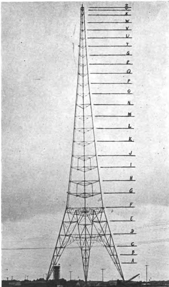
FIG. 2.—Lafayette Radio Station. Individual tower with panel points indicated.
