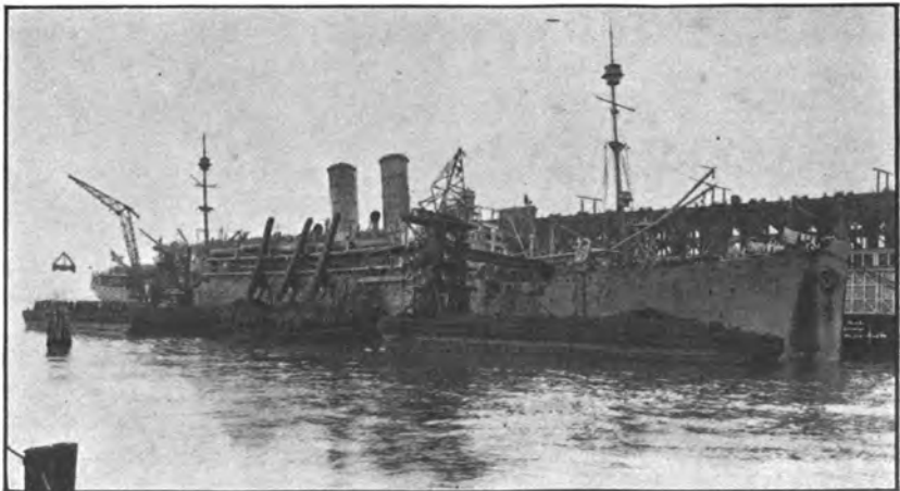
Mitchner elevators, stream fuelling barge, and escalade in operation at Bunkering Depot, Pier 4, Lamberts Point, Va.
