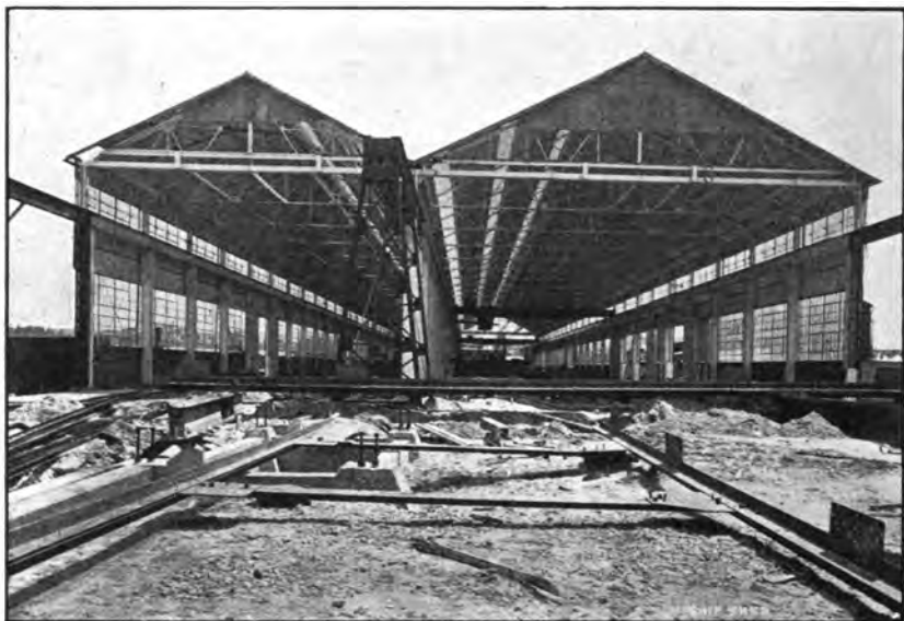
Ship fabricating shed, Navy extension to plant of Newport News Shipbuilding and Dry Dock Co., Newport News, Va.
