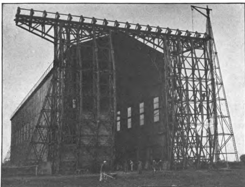
Frame dirigible hangar, United States Naval Air Station, Paimboeuf, France; late construction view.
